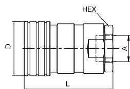
Female Thread
