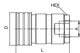
Female Thread
